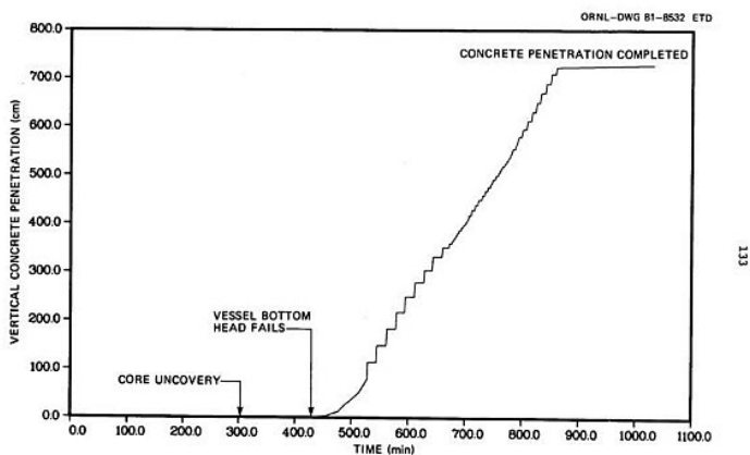
Fig. 9.21 Vertical concrete penetration.
