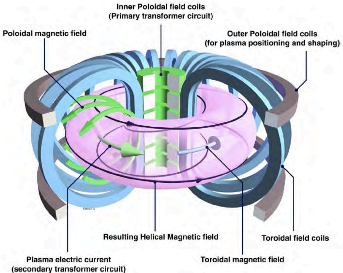
Figure 1.1: The tokamak [2]
