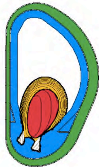
Figure 4.3-2 Plasma Current Density during a Downward VDE
